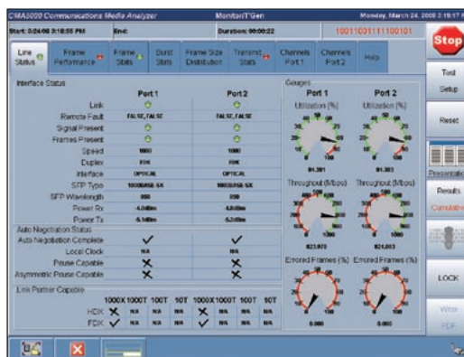
Measurement Results of Two Ports with User Adjustable Thresholds
