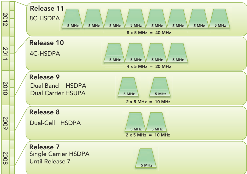
Figure 1 : Evolution of HSPA Carrier Aggregation
