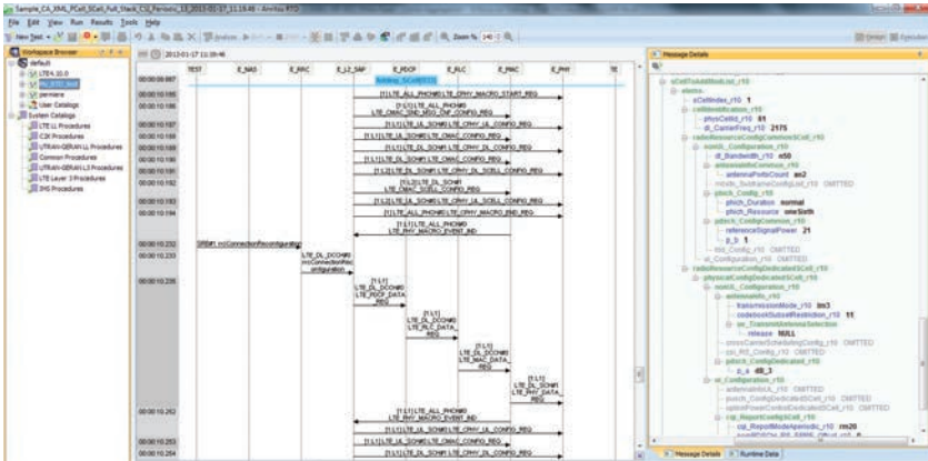
Figure 32: Example of SCell Addition Protocol flow
