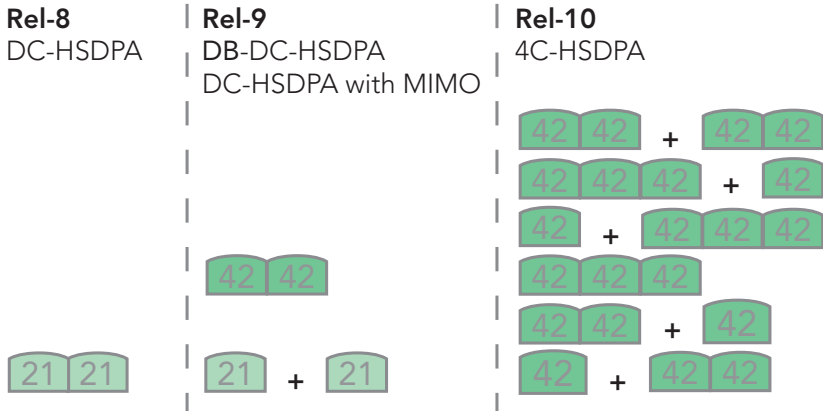
Figure 5 : Rel-10 4C-HSDPA Band combination
