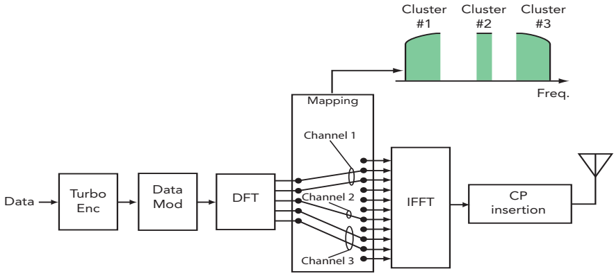
Figure 19 : Representation of clustered DFT-Spread-OFDDM
