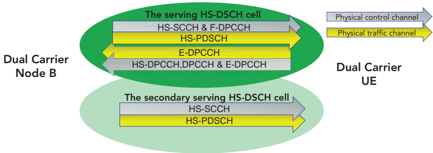
Figure 8 : Dual carrier channels mapping in DC-HSDPA
