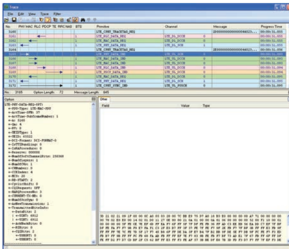
Figure 32: Example of SCell Addition Protocol flow
