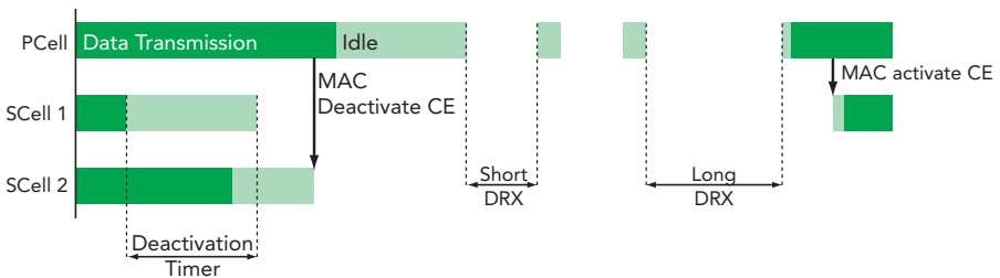
Figure 15 : SCell activation/Deactivation RRC timer
