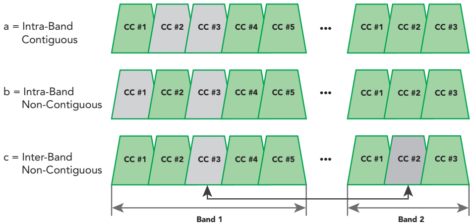
Figure 10 : Different type of CA allocation in LTE-A
