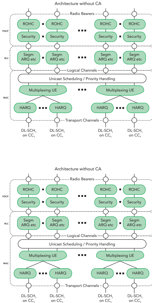
Figure 14 : Evolution of Architecture for LTE-A Carrier Aggregation
