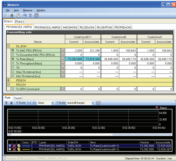
Figure 34: Throughput testing category UE LTE Cat 6 - 2CC of 10 MHz - 2x2 MIMO
