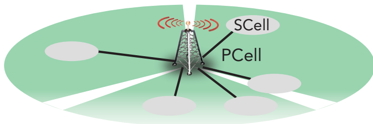
Figure 16 : Non co-located site, carrier aggregation
