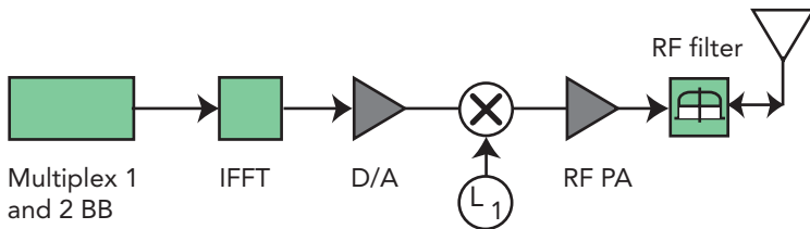
Single (baseband + IFFY + DAC + mixer + PA)
